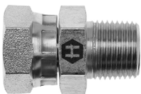
H9205X2X2 ADAPT FEM NPT TOURNANT X MALE NPT 1/8 ADAPT FEM NPT SWIVEL X MALE NPT 1/8
